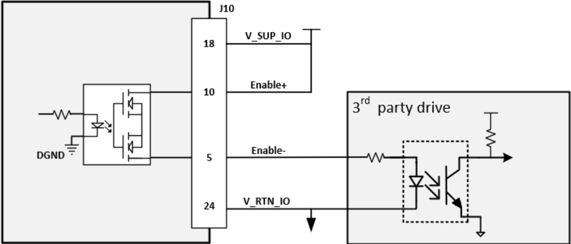
Figure 4-6. Drive Enable of P/D module (axis 5)
