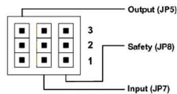
Figure 8-8. Sink or Source Jumper Configuration
