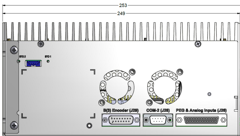
Figure 12-2. SPiiPlusCMxa Side
