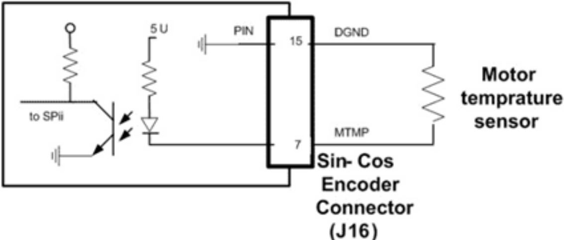
Figure 8-6. Motor Over Temperature Connection
