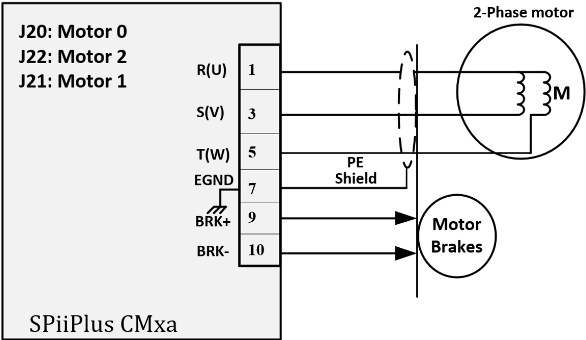
Figure 3-3. 2-Phase Step Motor Connection
