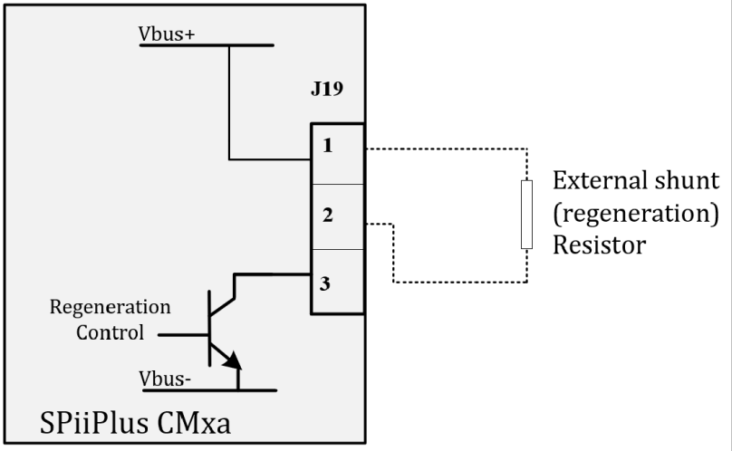
Figure 3-5. External Regeneration Connection
