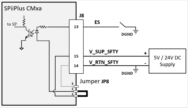
Figure 8-4. Emergency Stop (Sink) schematic diagram
