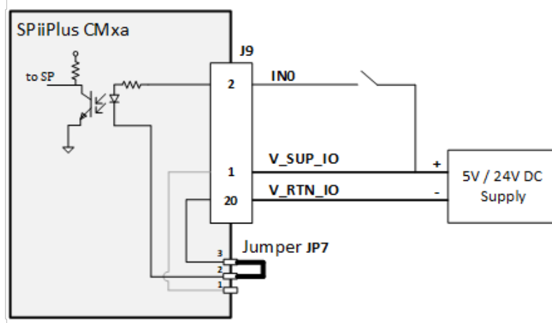
Figure 6-3. Source Digital Inputs
