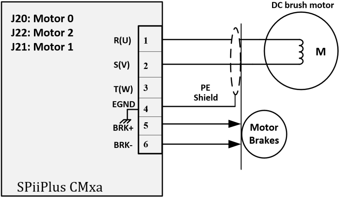
Figure 3-2. DC Brush Motor Connection
