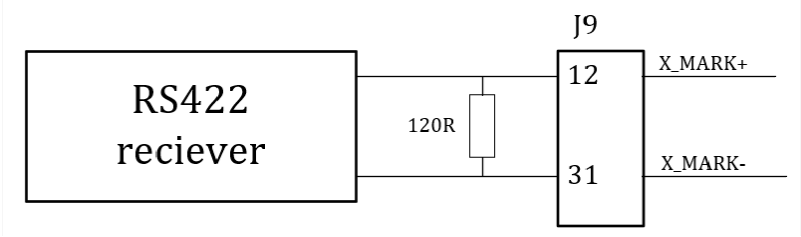
Figure 6-5. Differential Connection for MARK1 Input
