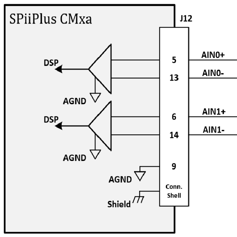
Figure 7-1. General Purpose Analog Inputs
