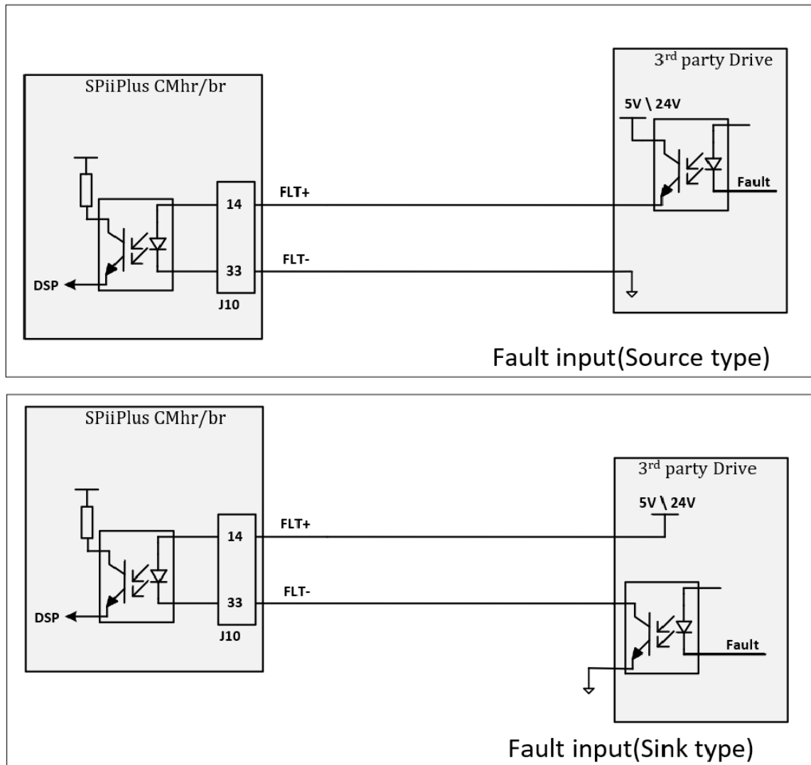
Figure 4-7. Fault signal electrical schematic, 'source' and 'sink' connectivity scheme.
