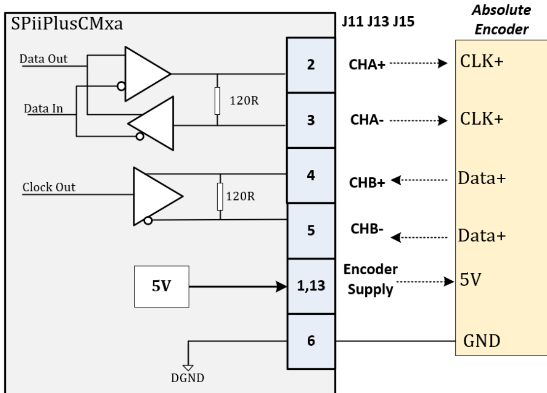
Figure 4-2. Sin-Cos Encoder Connections
