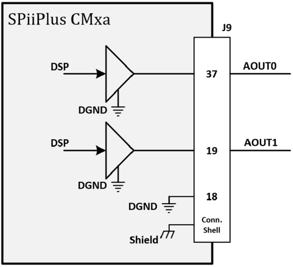
Figure 7-2. Analog output schematic diagram
