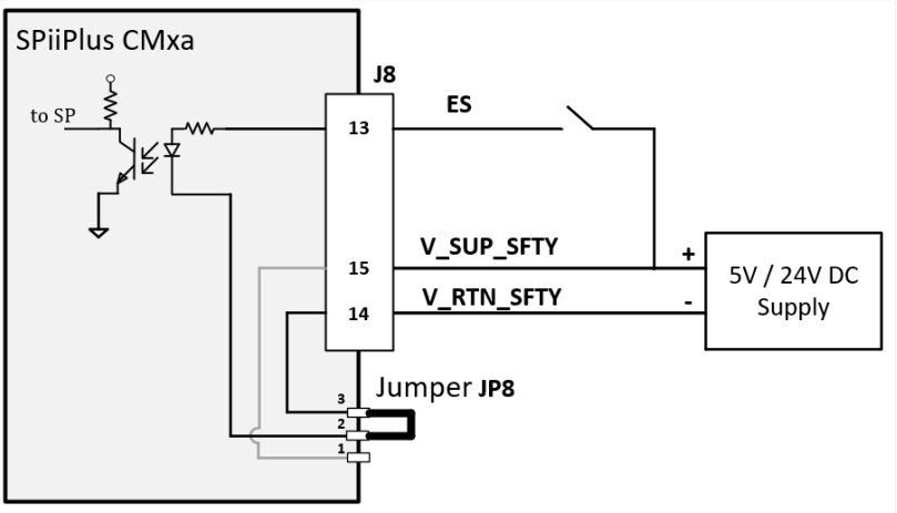
Figure 8-3. Emergency Stop Source Input
