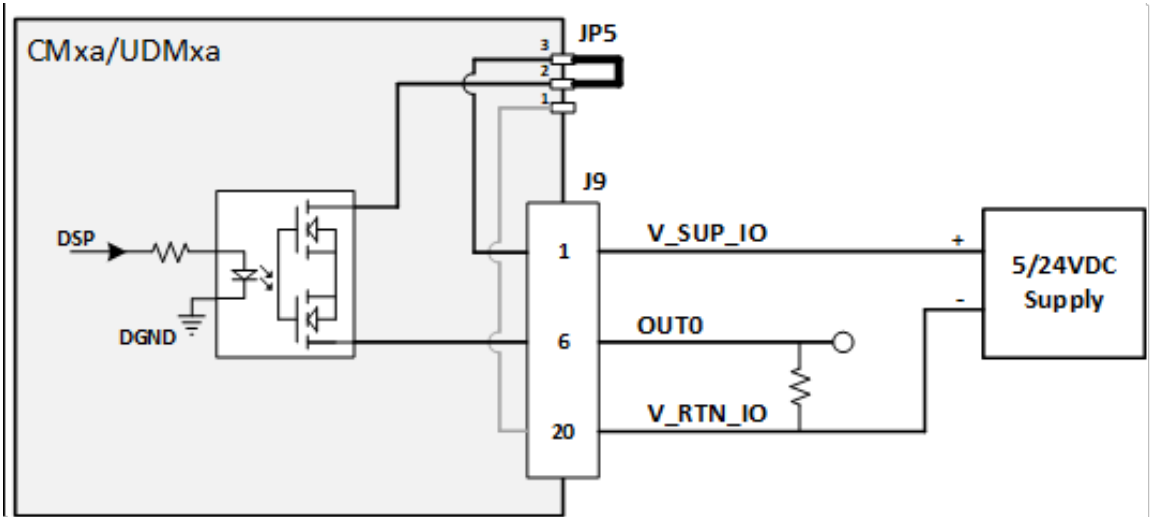
Figure 6-1. Digital Output Connection (source)
