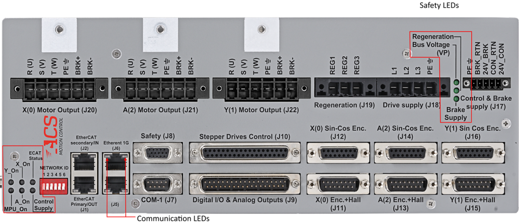
Figure 2-5. SPiiPlusCMxa LED Indicators
