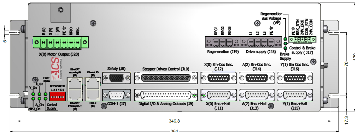
Figure 12-1. SPiiPlusCMxa Front
