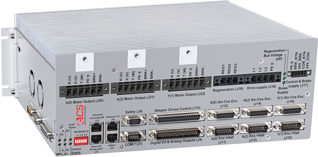
Figure 2-4. Connectors on Front and Side Panels
