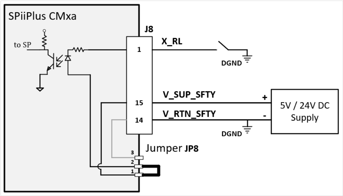
Figure 8-2. Right Limit (Sink) schematic diagram
