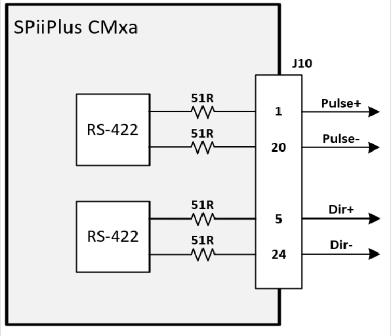
Figure 4-5. Pulse and Direction electrical schematic
