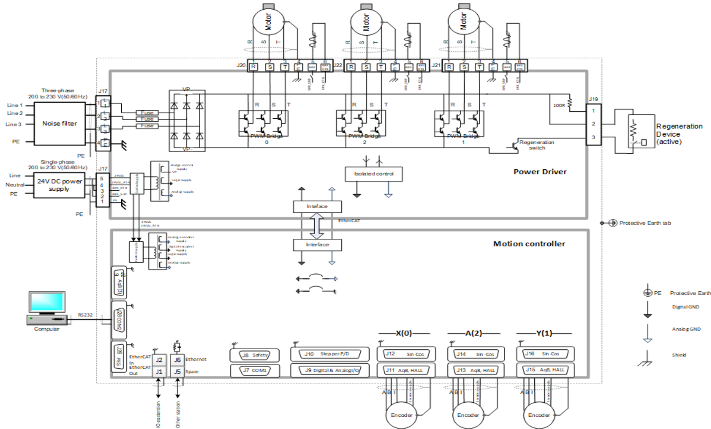
Figure 10-1. Grounding and Shielding
