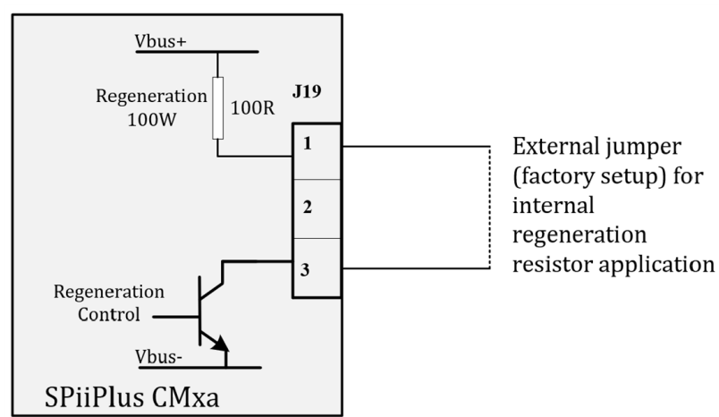
Figure 3-4. Internal Regeneration Connection
