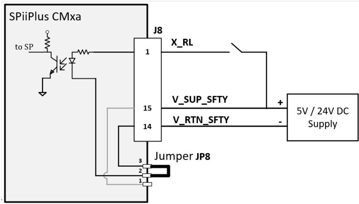
Figure 8-1. Right Limit (Source) schematic diagram
