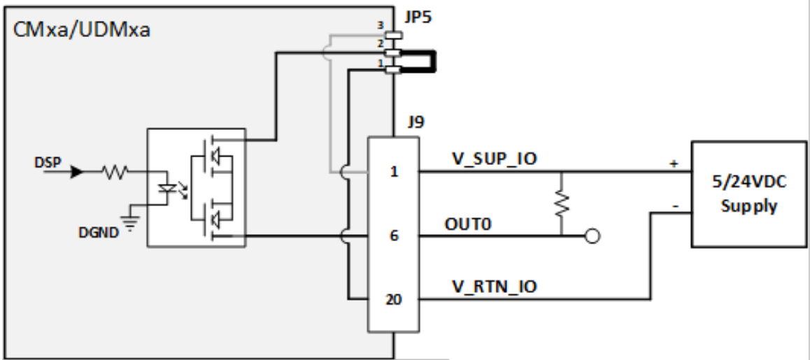
Figure 6-2. Digital Output Connection (sink)
