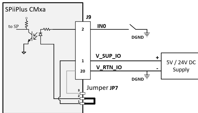
Figure 6-4. Sink Digital Inputs
